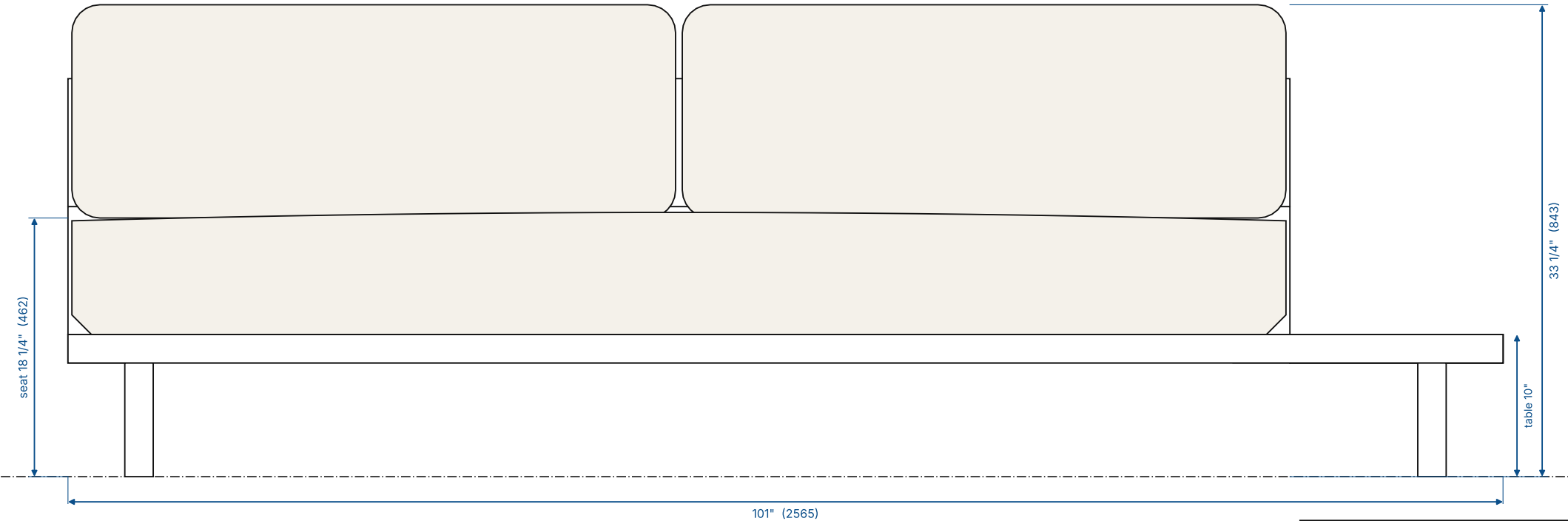
FRONT ELEVATION 1:10
